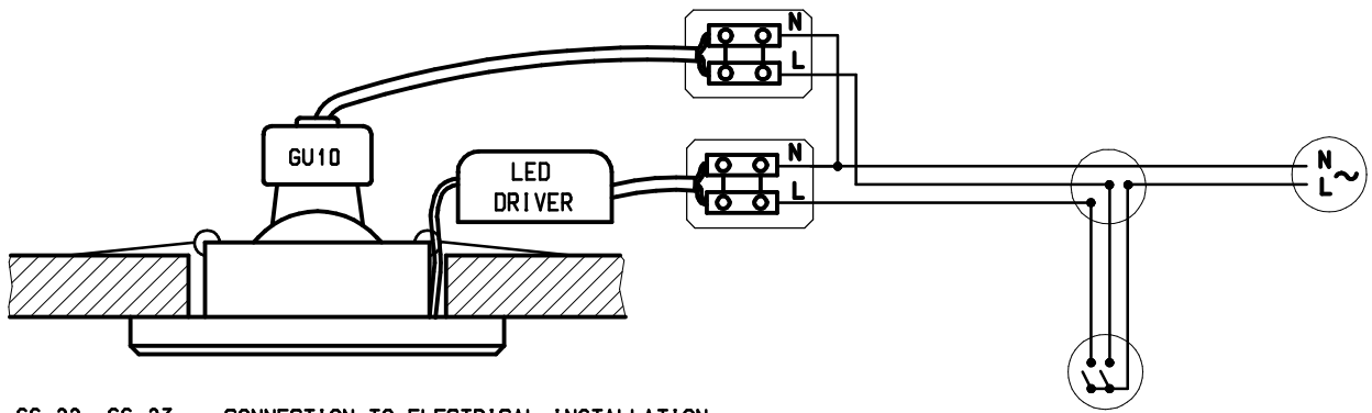
SS-22. SS-23 CONNECTION TO ELECTRICAL INSTALLATION
